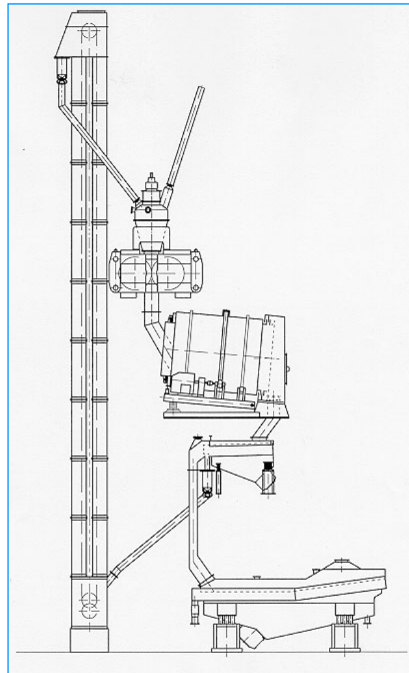
Figure 7: Briquetting line for hot sponge iron fines with drum separator.
