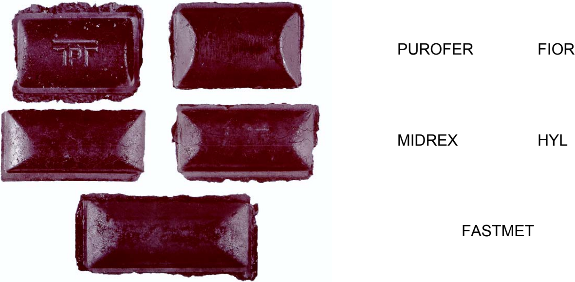
Figure 8: Briquettes made of product from different direct reduction processes by hot briquetting.
