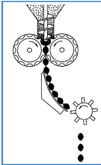
Figure 3: Typical schematic of hot briquetting.
