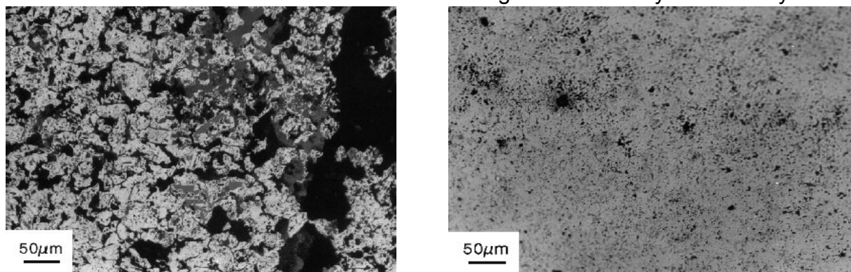
Figure 1: Comparison of the structure of DRI pellets (left) and HBI (right).
