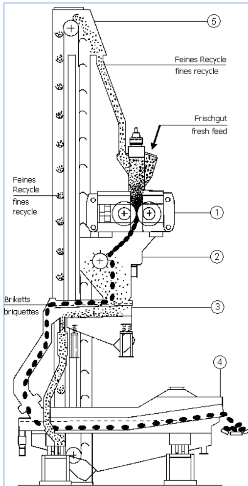
Figure 6: Flowsheet of a briquetting line for hot sponge iron from lump ore and pellets.
