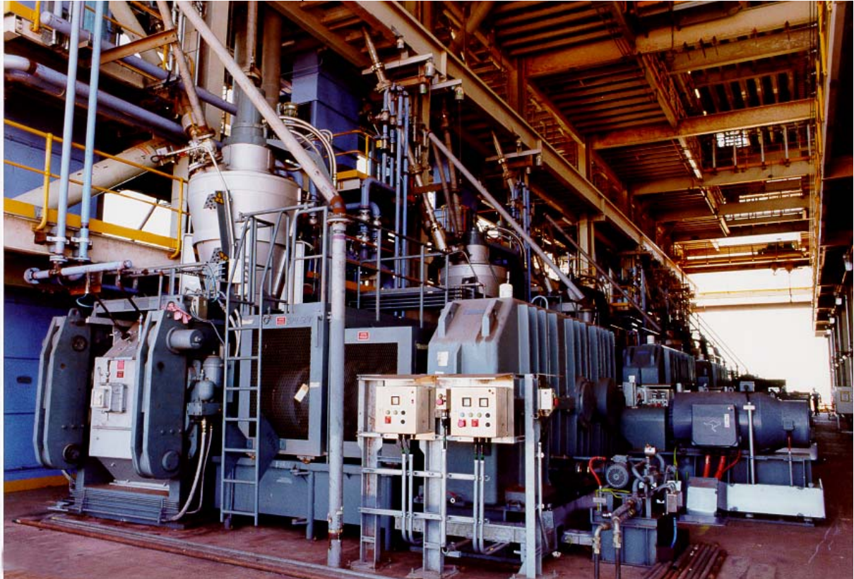
Figure 5: Briquetting machine for the production of HBI from fine ore. Roller diameter 1,400 mm.
